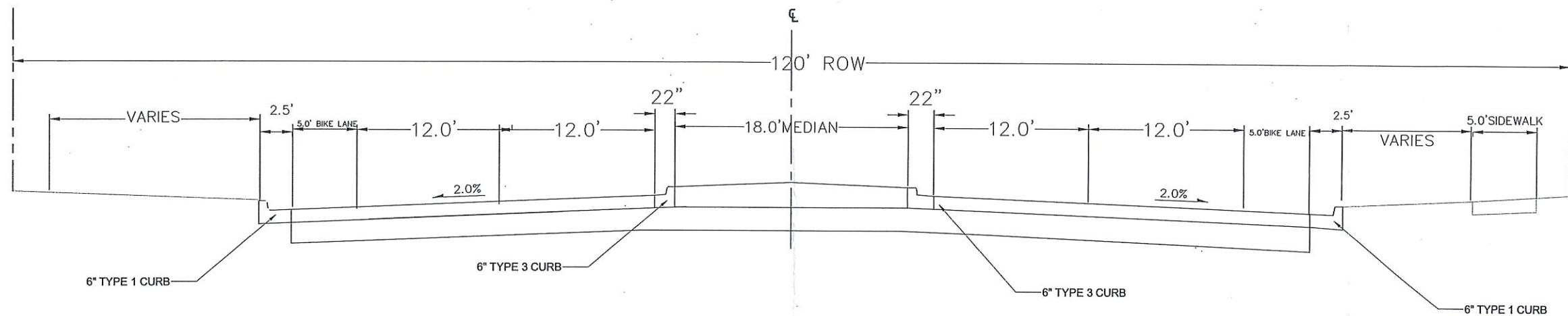
TYPICAL SECTION JACKSON CREEK PARKWAY
